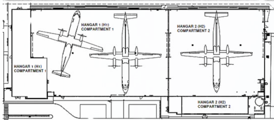
1 GROUND FLOOR - AIRCRAFT OPTION 1 1:500
