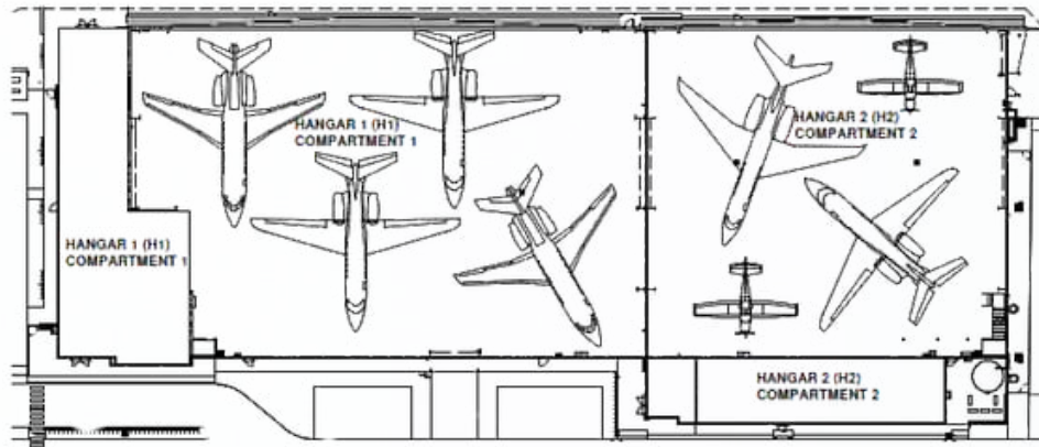
3 GROUND FLOOR - AIRCRAFT OPTION 3 1:500
