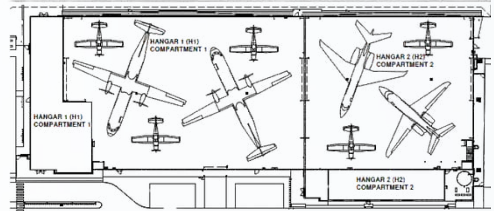
2 GROUND FLOOR - AIRCRAFT OPTION 2 1:500
